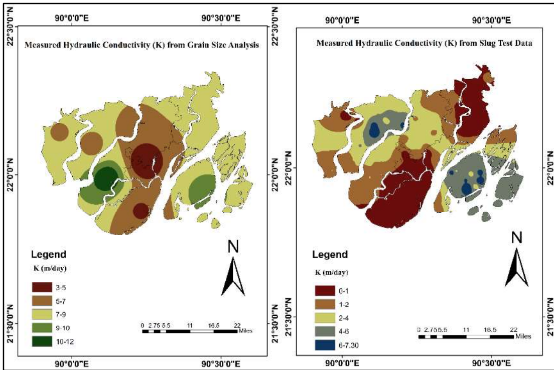
Figure 3: Hydraulic Conductivity measured using different methods
