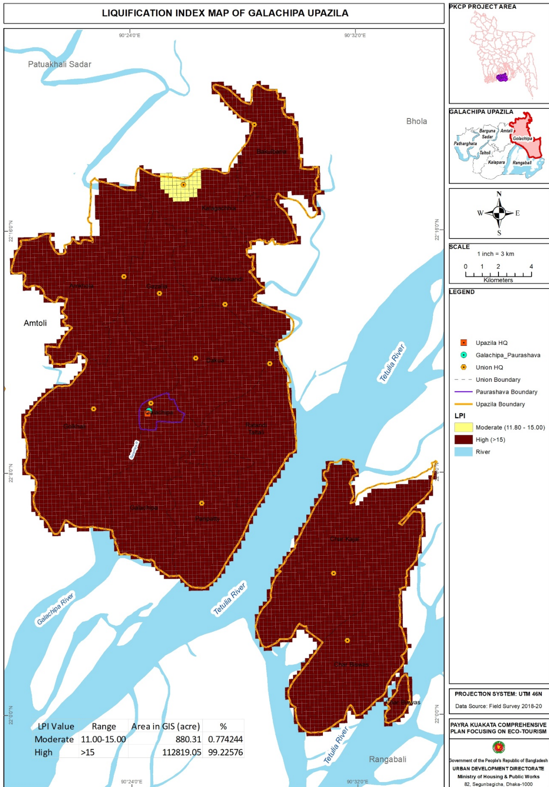
Figure 31: Liquefaction Potential Index map of Study Area
