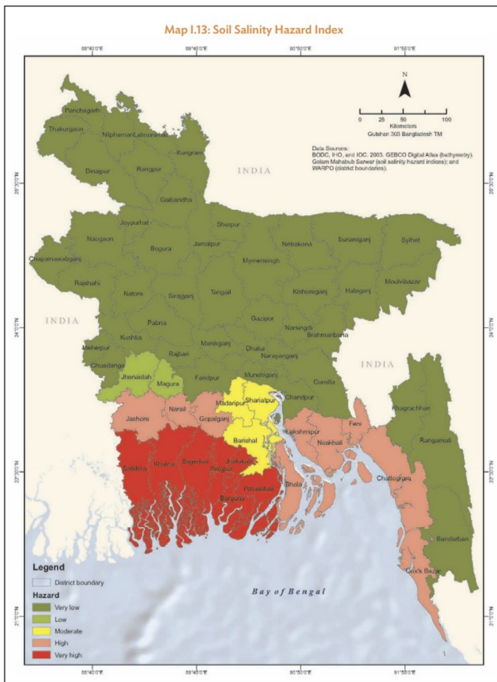
Figure 13 Soil Salinity hazard map of the coastal zone in Bangladesh [Source: ADB, 2021]
