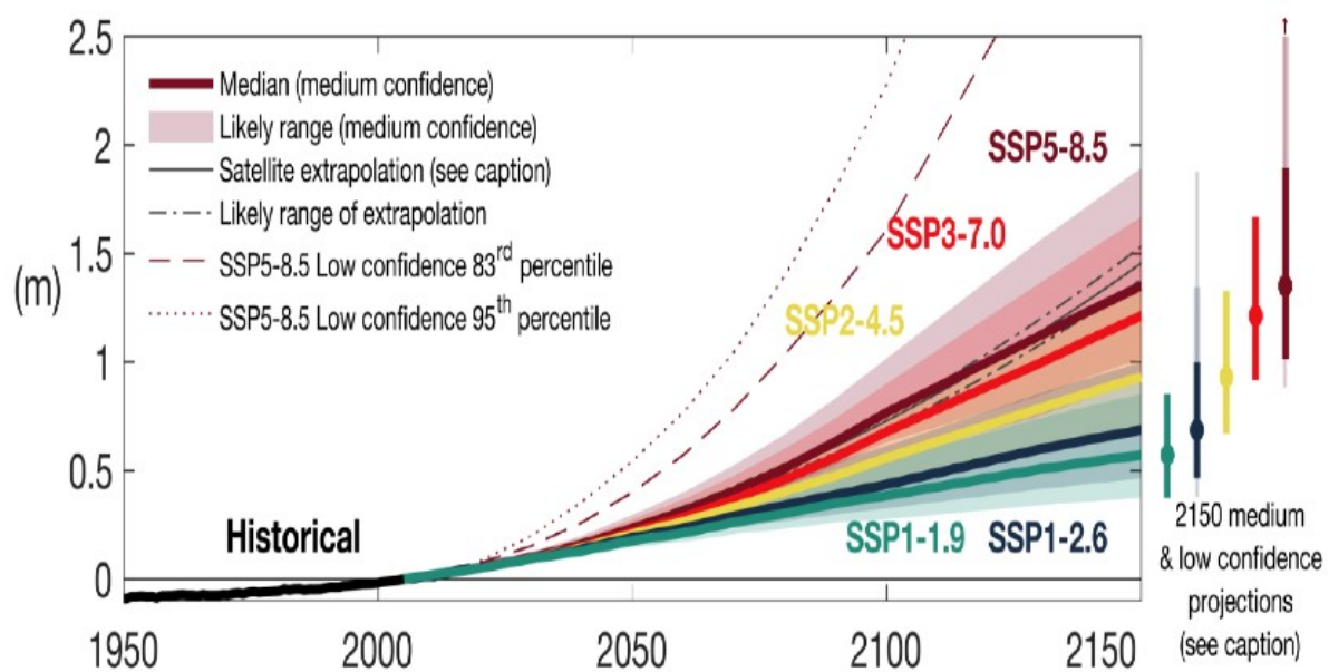
Figure 14 Projected global mean sea level rise (m) under different SSP-RCP scenarios based on CMIP6 models (Arias et al., 2021).
