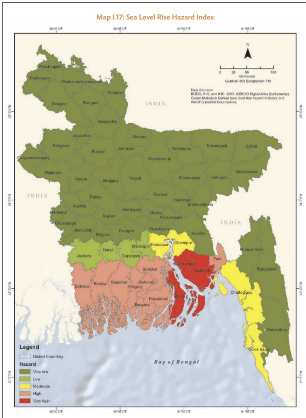
Figure 16 Sea Level Rise hazard map of the coastal zone in Bangladesh [Source: ADB, 2021].
