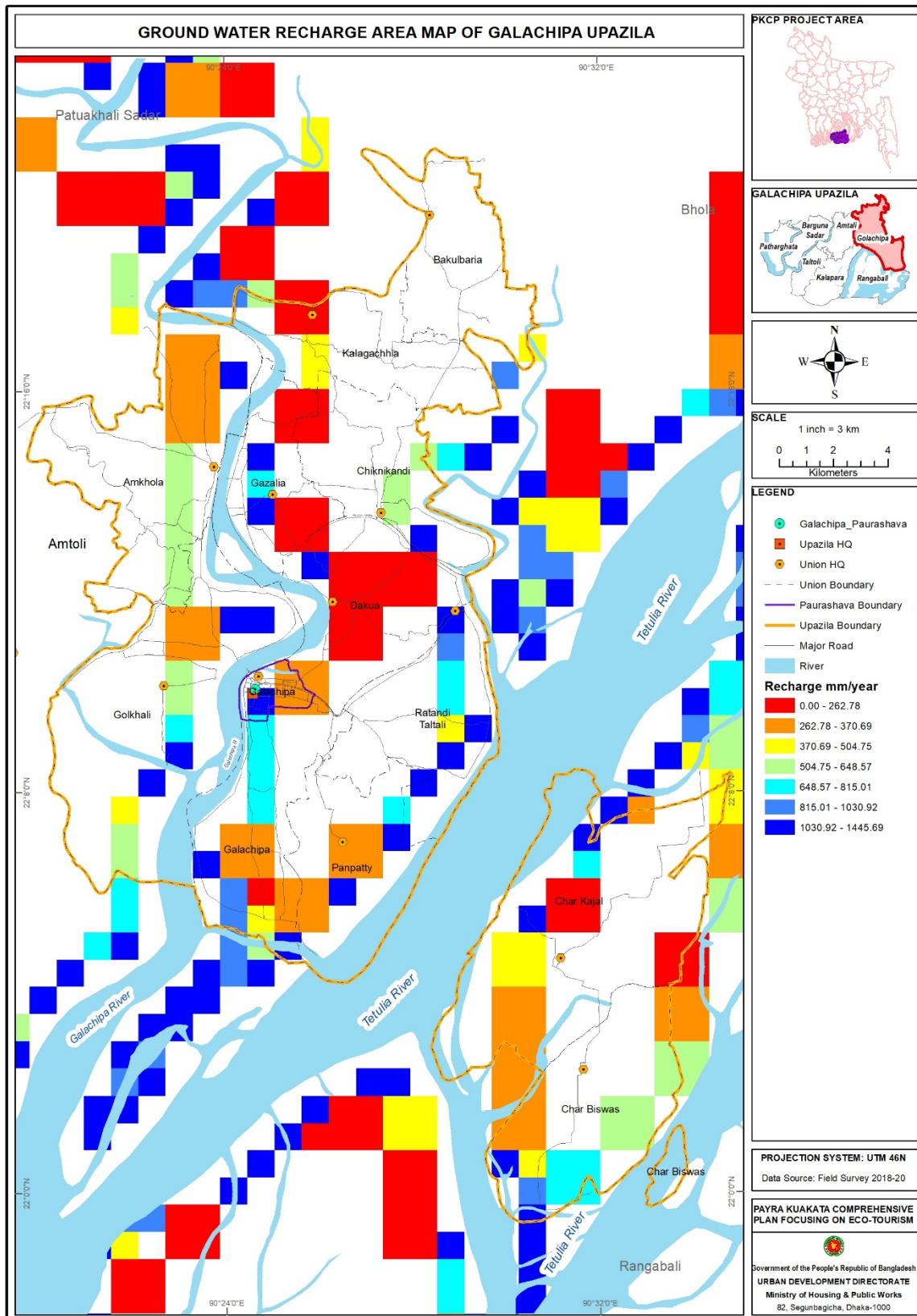
Figure 26: the model simulated actual recharge in GalachipaUpazila in 2019
