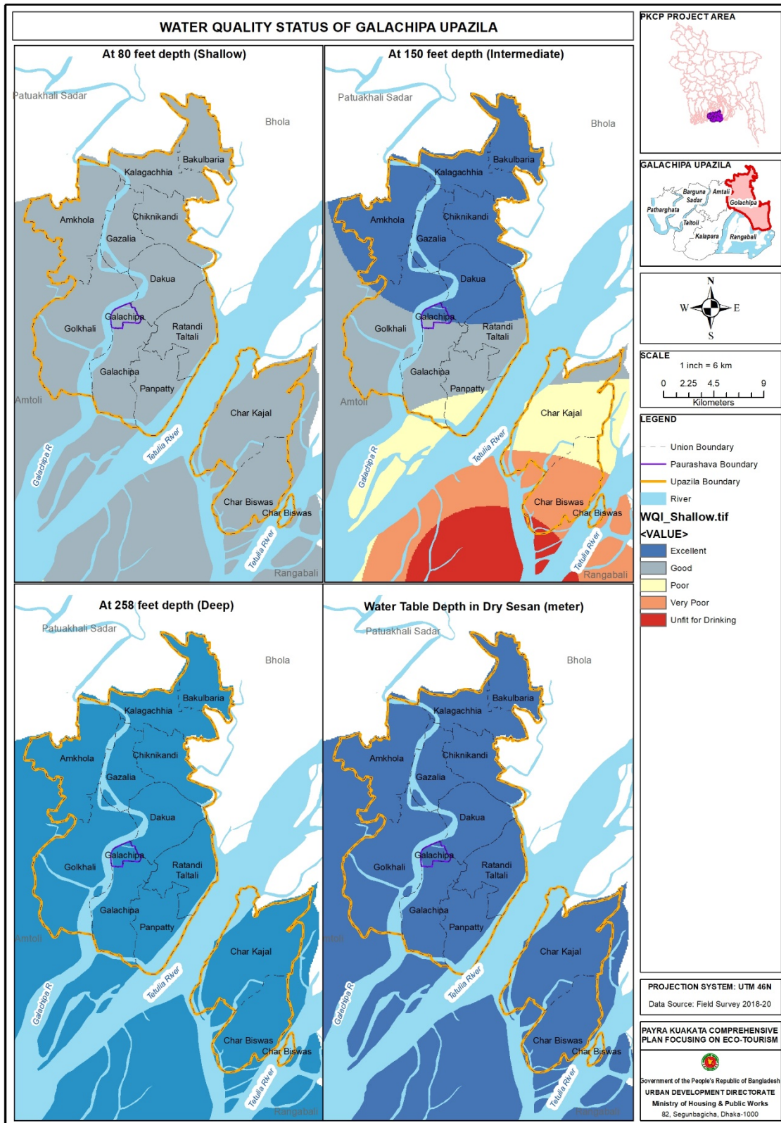
Figure 25: WQI of shallow, intermediate and deep aquifer
