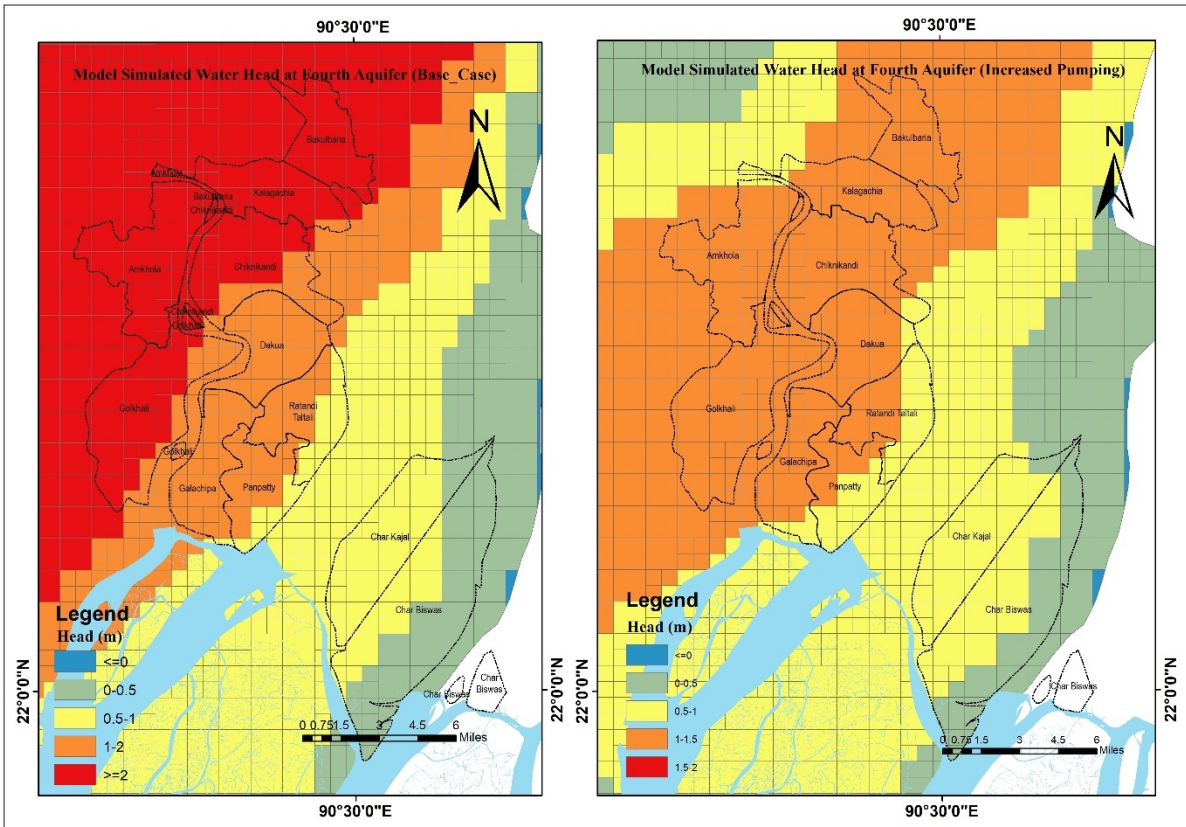
Figure 10: comparison between deep aquifer in Base Case condition in December 2019 (left) and in increased pumping condition in December 2025 (right)
