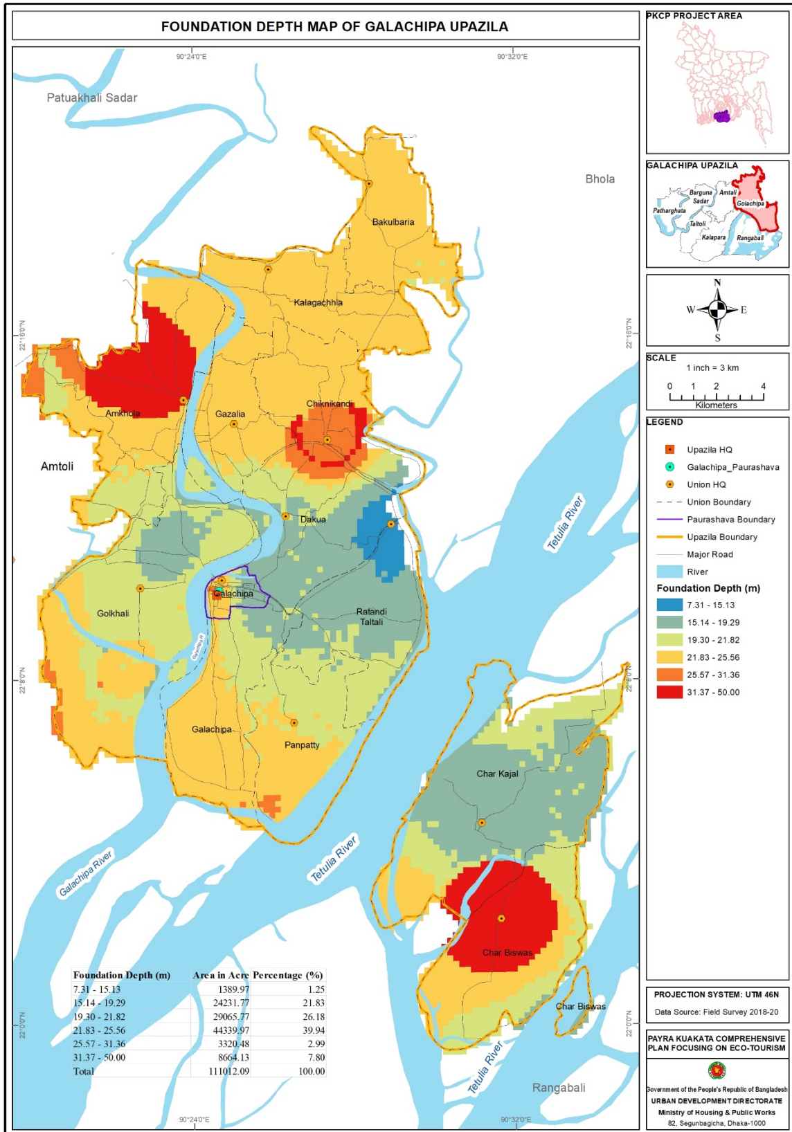
Figure 27: Foundation layer depth map
