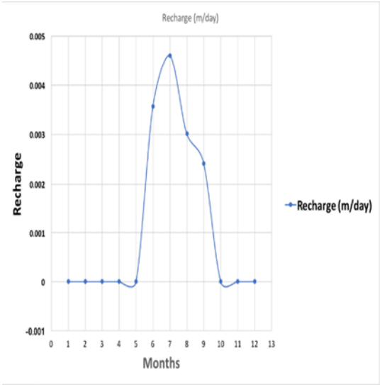
Figure 37 : Potential recharge measured by Chaturvedi (1973) formula
